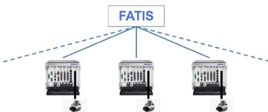
Figure 1: FATIS Scalability
